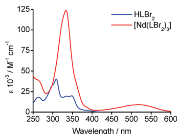
Figure 4. Absorption spectra of the ligand HLBBr 2 ( 1.77 \times 10^{-4} M) and its Nd III complex ( 3.85 \times 10^{-5} M) in CH 2 Cl 2 solution. Absorption spectra for other ligands and complexes are provided in the Supporting Information.
